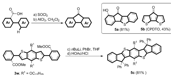
Scheme 5. Transformations of ortho -carboxy-substituted bi(hetero)aryls into various cyclopentadiene derivatives ( 5 ). THF = tetrahydrofuran.
